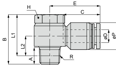
Appearance dimension for taper pipe thread (R)
