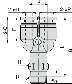
Appearance dimension for taper pipe thread (R)
