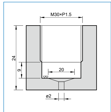
Mounting diagram
