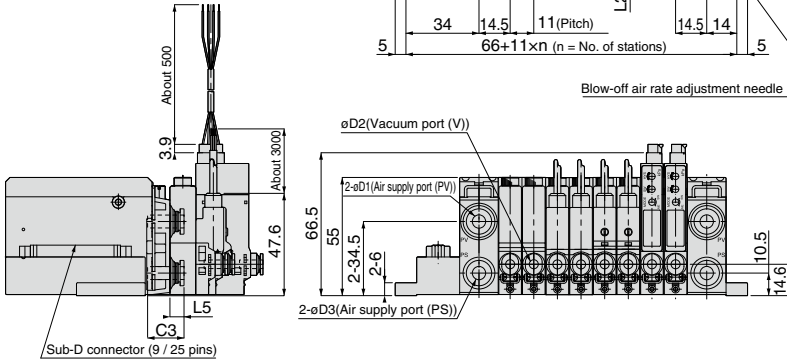
Dimension of Fitting
